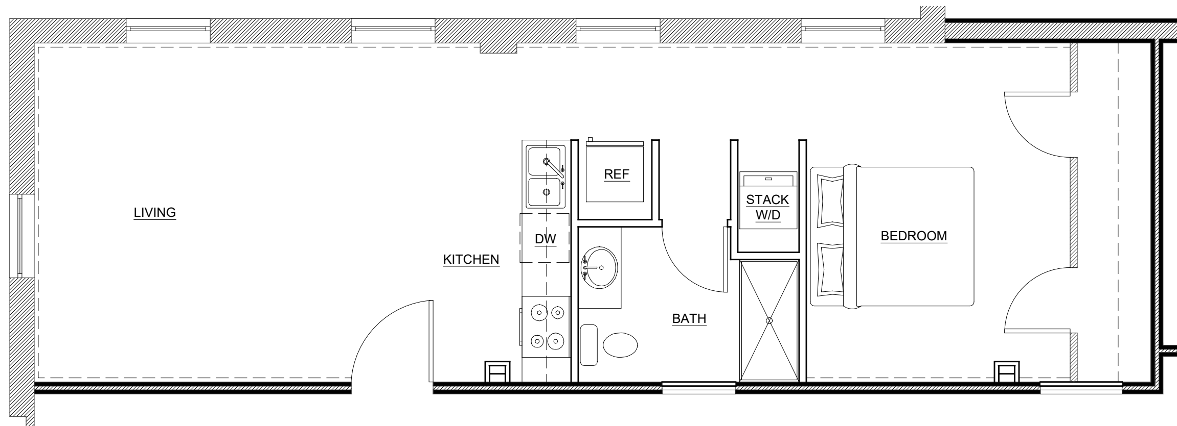
UNIT #102 - 1 BD / 1 BA / 629 SF
